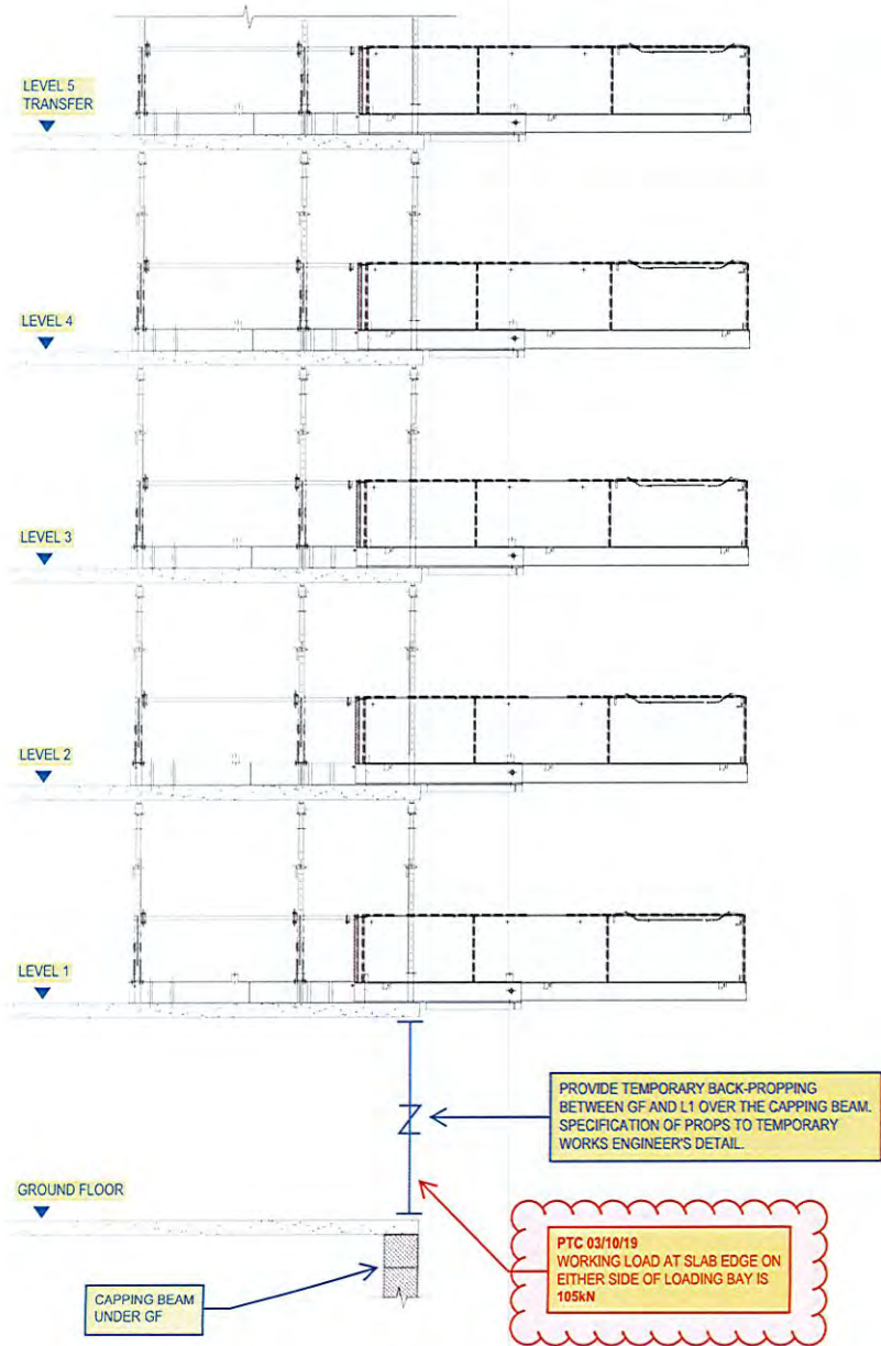
SECTION 1 LOADING BAYS INSTALLED ON L1 TO L4
