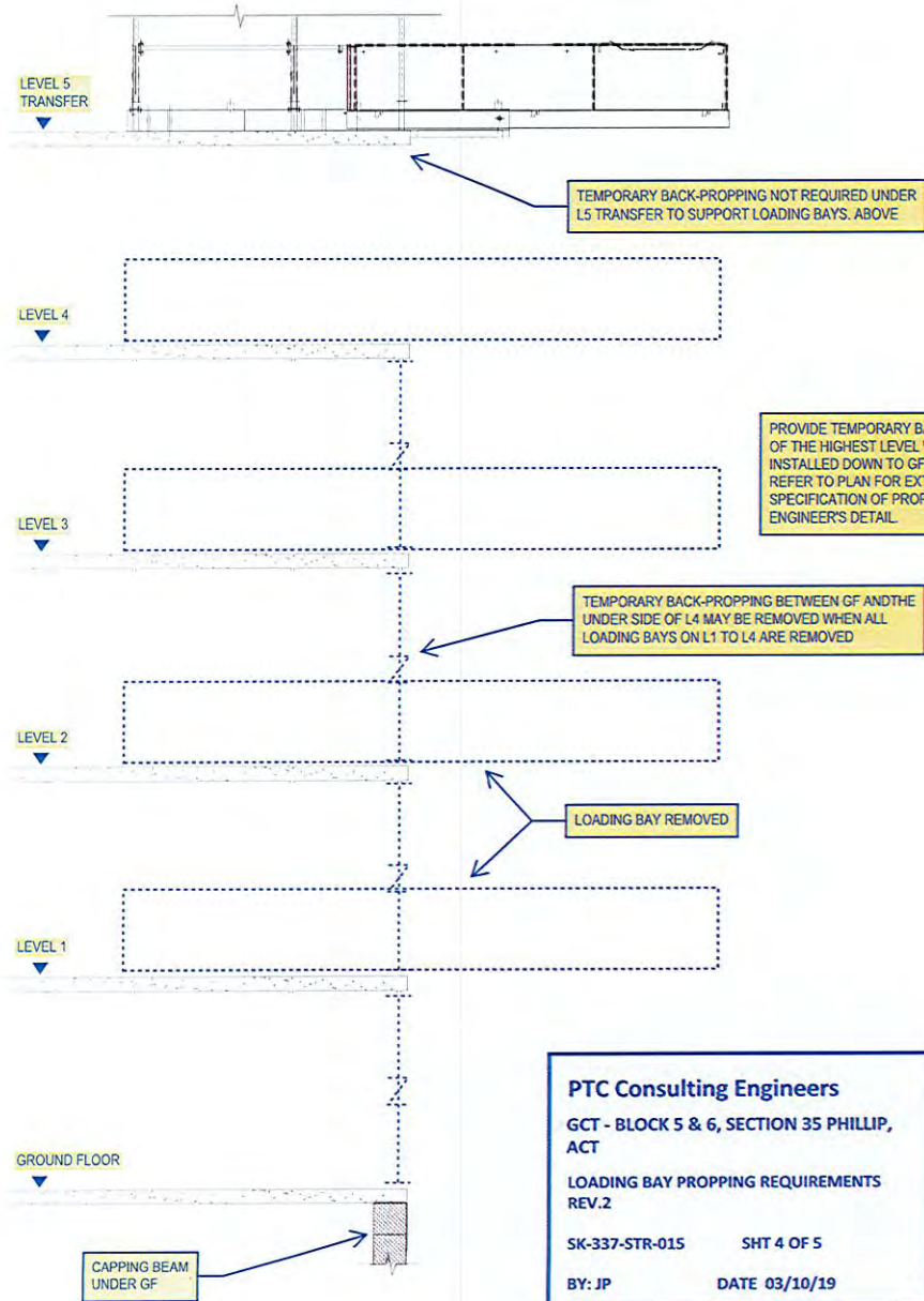
SECTION 1 LOADING BAYS REMOVED BETWEEN L1 TO L4
