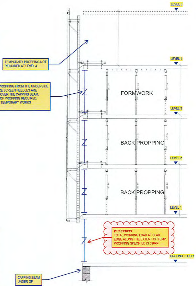
SECTION 2 TEMPORARY BACK-PROPPING BETWEEN GRID 6 & 7 SCREEN NEEDLES INSTALLED AT L4 AND BELOW
