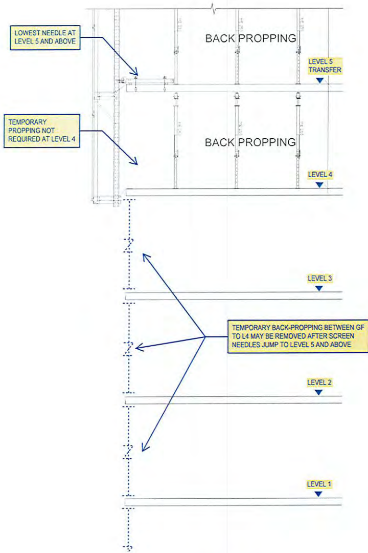
SECTION 2 TEMPORARY BACK-PROPPING BETWEEN GRID 6 & 7 SCREEN NEEDLES INSTALLED AT L5 AND ABOVE
