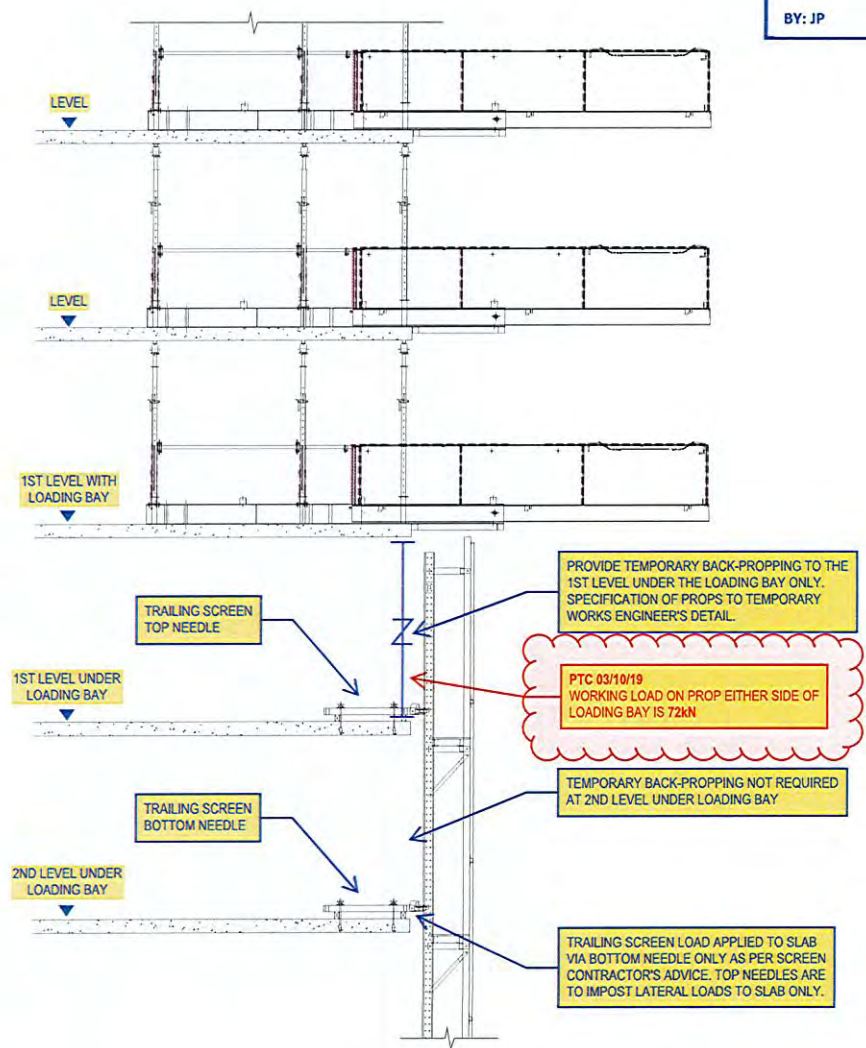
SECTION 3 TYPICAL BACK-PROPPING UNDER FIRST LOADING BAY
