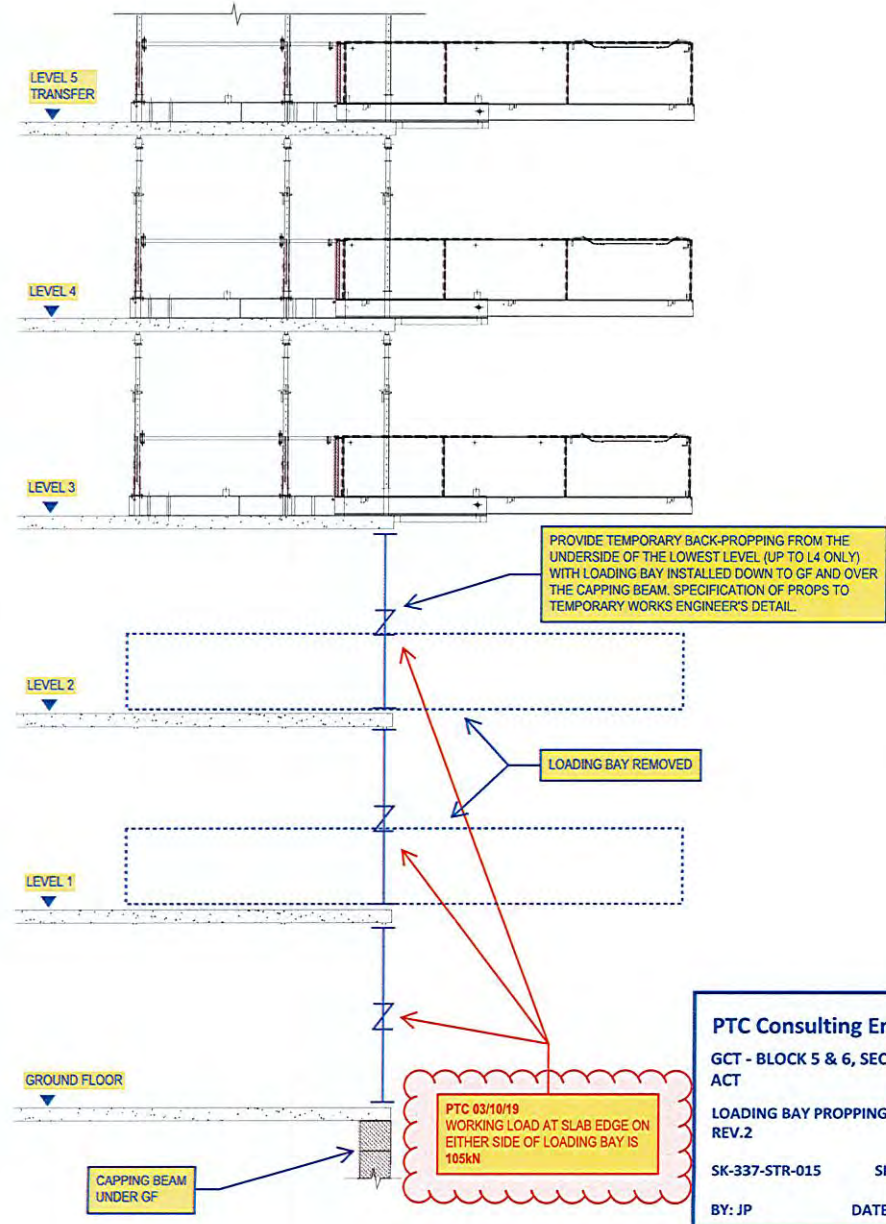
SECTION 1 LOADING BAYS REMOVED AT LOWER LEVELS
