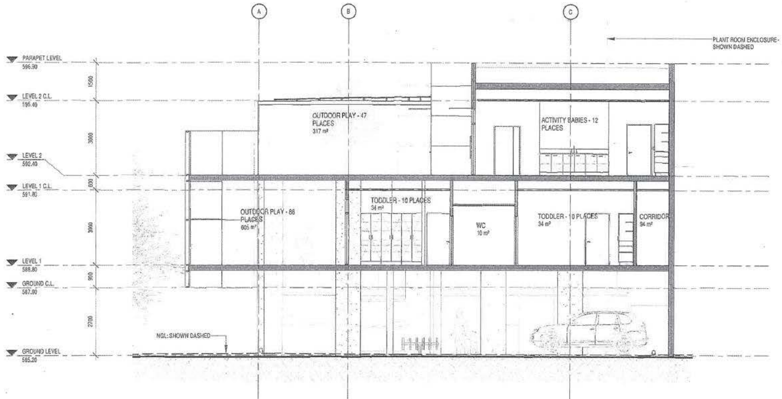
1 SECTION A 102 1:100
