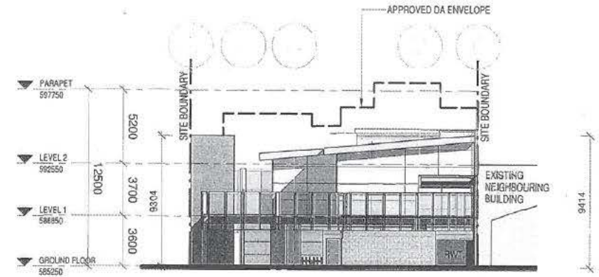
2 WEST ELEVATION 1 : 250
