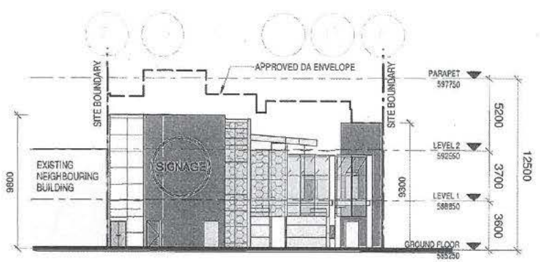
1 EAST ELEVATION 1 : 250
