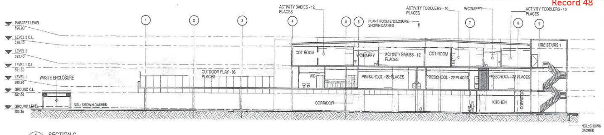
1 SECTION C 102 1:250
