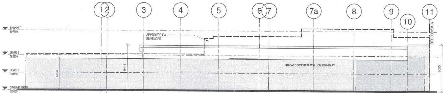
2 SOUTH ELEVATION 1 : 250
