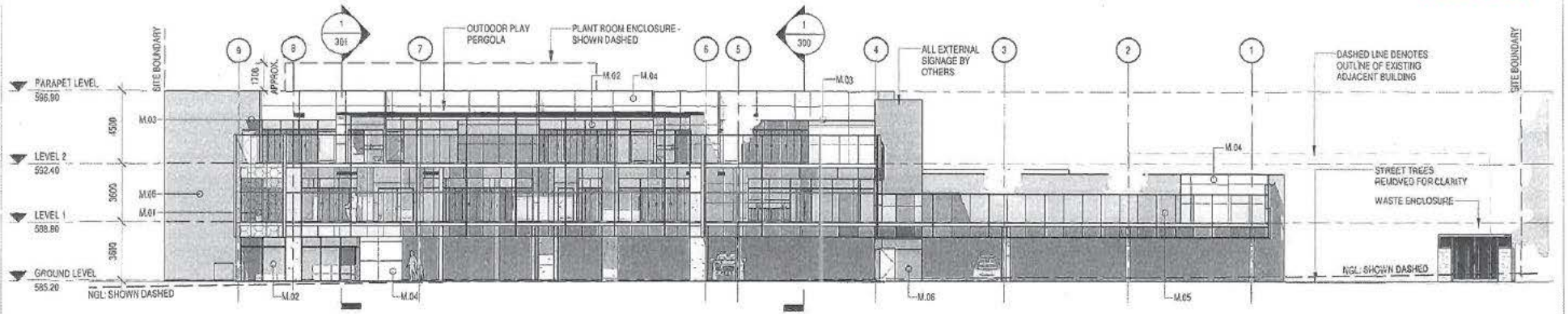
1 NORTH ELEVATION 102 1:250
